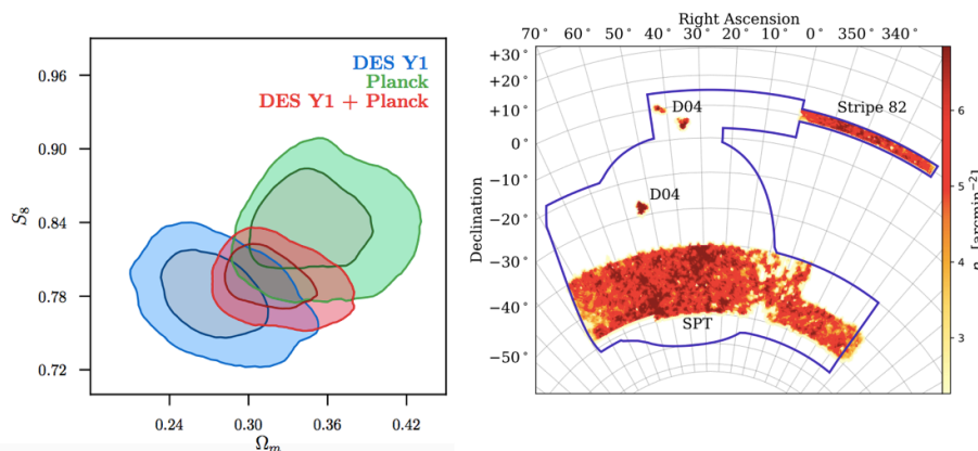
Figure 5: Left: First year DES constraints on the dark matter density of the Universe ( \Omega_m ), vs. the clumpiness of dark matter ( S_8 ), derived from galaxy clustering and weak lensing (blue contours). These are compared to, and combined with, Planck results (DES collaboration 2017, Phys Rev D , 98, 042536). Right: the galaxy areal density for the DES year 1 survey (Zuntz et al. 2017, MNRAS ).
