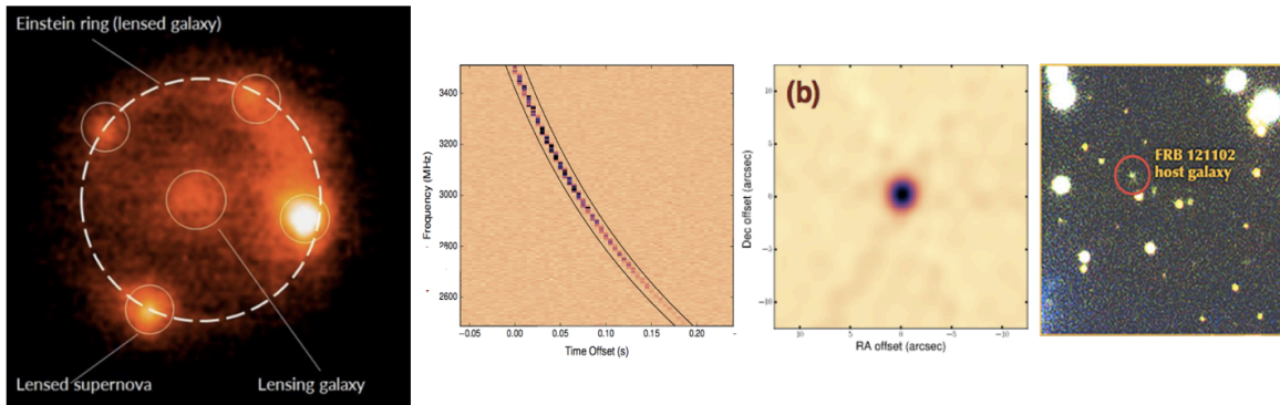
Figure 4: Left: The strongly lensed images of a type Ia Supernova at z = 0.4 seen by the GROWTH survey (Goobar et al. 2017, Sci , 799, 106). Right: Arecibo discovered a repeating Fast Radio Burst, which then was localized by the JVLA to an arcsecond. Subsequent optical follow-up associated the source with a low metallicity dwarf galaxy at z = 0.2 (Tendulkar et al. 2017, ApJ , 834, 7; Chatterjee et al. 2017, Nat , 541, 58).
