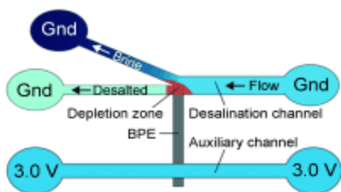
Figure 4. A bipolar electrode drives electrolysis reactions to create an electric field gradient that directs salt into one branch of a microfluidic network.
