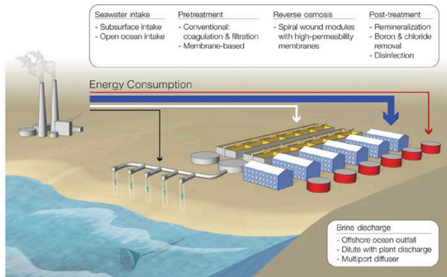
Figure 3. Conceptual drawing of an SWRO desalination plant showing the various stages—seawater intake, pretreatment, reverse osmosis, post-treatment, and brine discharge—and their interactions with the environment. The thickness of the arrows represents the relative amount of energy consumed at the various stages.
