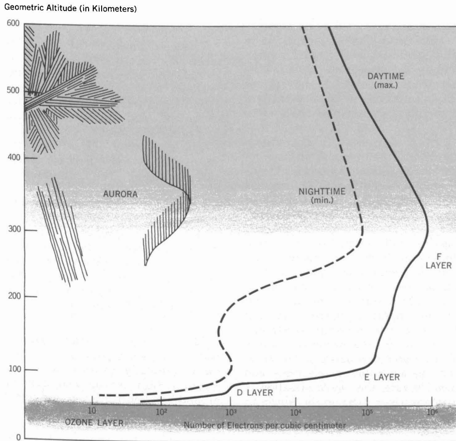
Figure I-4 — THE IONOSPHERE
