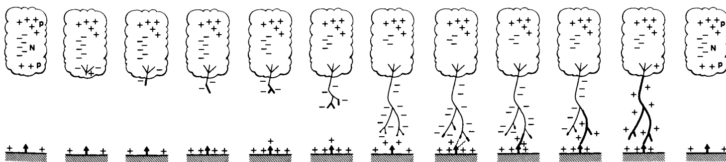
Figure V-15 — THE INITIATION OF A LIGHTNING STROKE
