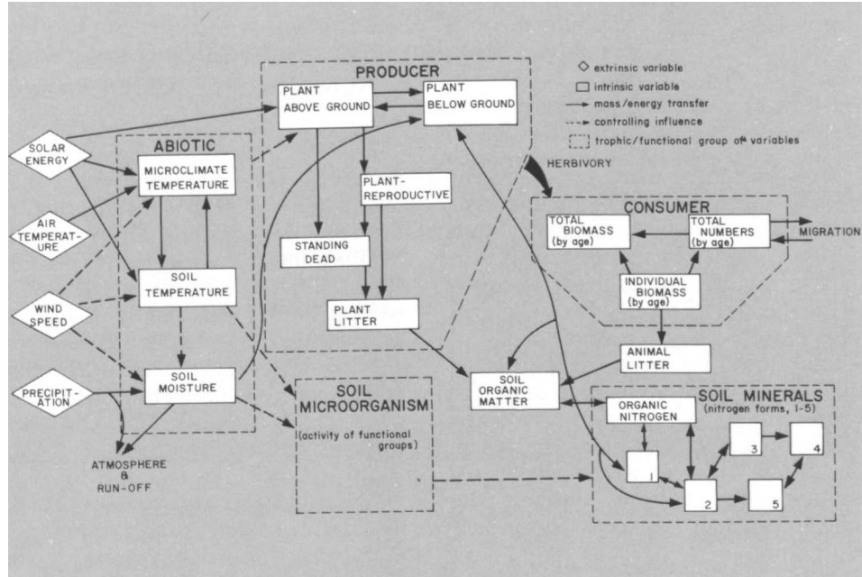
Figure IX-2 — A SYSTEMS MODEL FOR A GRASSLAND ECOSYSTEM
