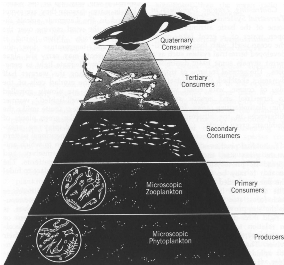
Figure VIII-1 — TROPHIC LEVELS
