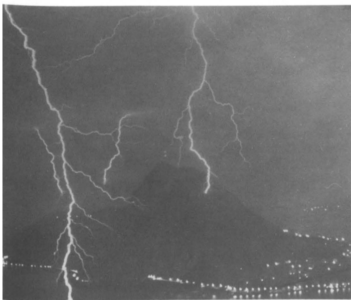
Figure V-14 — LIGHTNING
