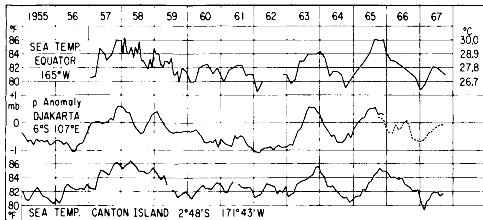
Figure IV-5 — WALKER'S "SOUTHERN OSCILLATION"
