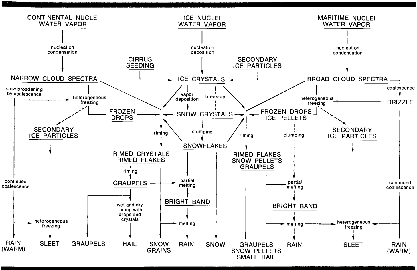
Figure VI-2 — PRECIPITATION PROCESSES
