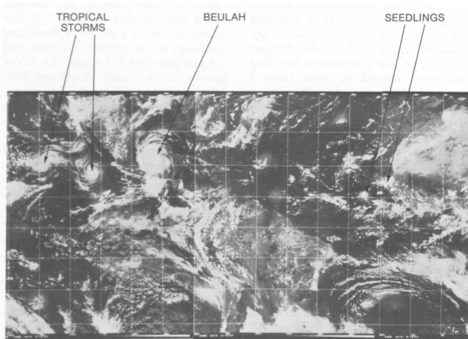
Figure V-2 — HURRICANE BEULAH, 1967
