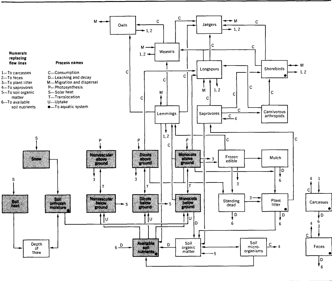
Figure IX-16 — FLOW DIAGRAM OF A WET COASTAL TUNDRA ECOSYSTEM
