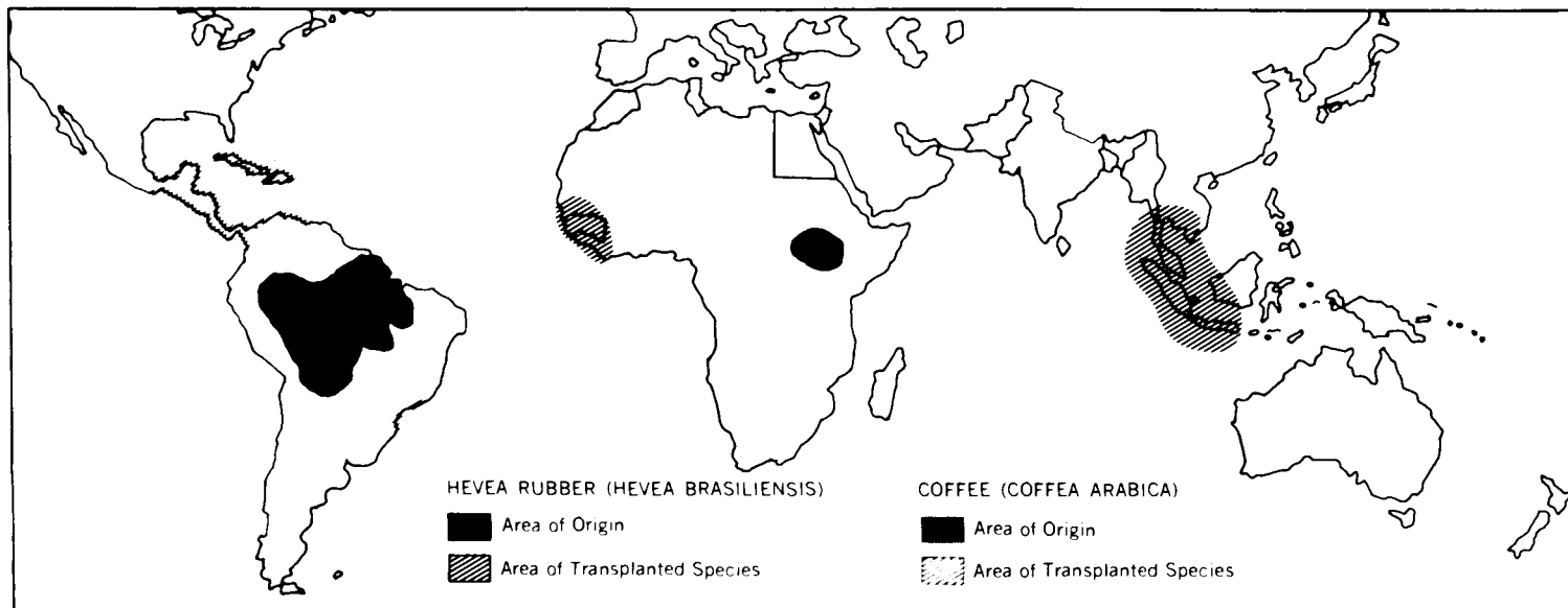
Figure VII-9 — TRANSPLANTED SPECIES
