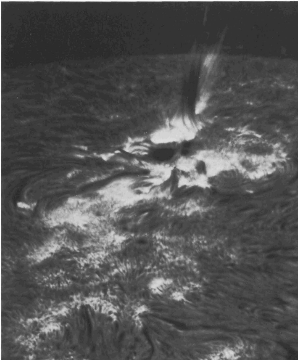
Figure I-1 — SOLAR FLARE
