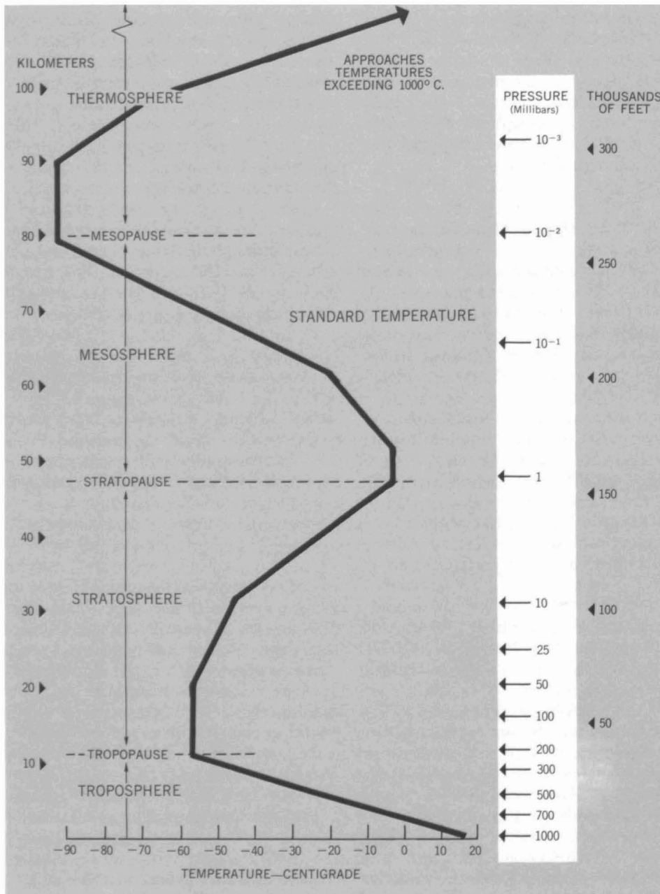
Figure 1-5 — ATMOSPHERIC TEMPERATURE DISTRIBUTION
