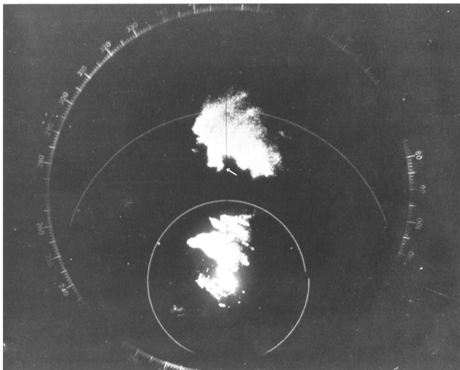
The picture is of a Plan Position Indicator (PPI) presentation of a severe storm over Oklahoma City on May 26, 1963. Range marks denote intervals of 20 nautical miles. North is toward the top. The radar is located at the center of the range circles. The arrow points out the location of the tornado.
