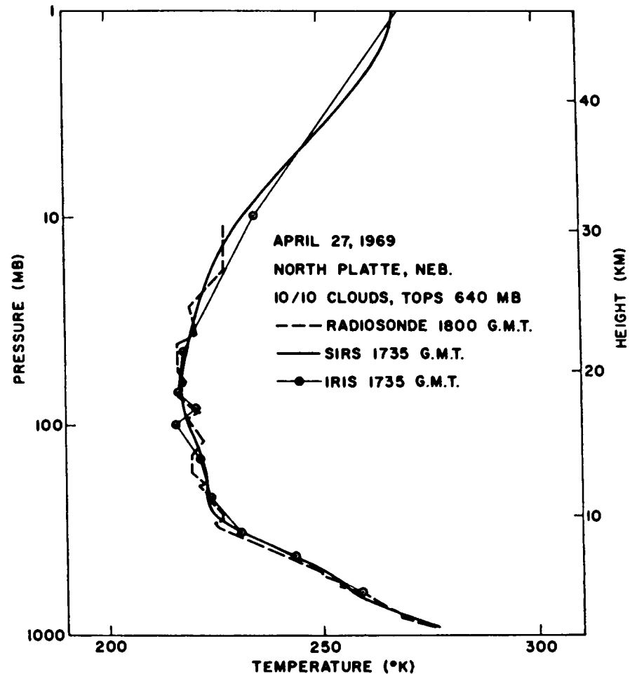
Figure IV-6 — SIRS SOUNDING
