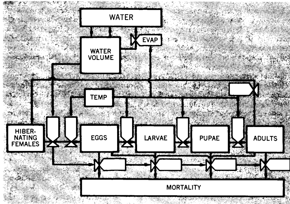
Figure IX-3 — MOSQUITO SUBMODEL
