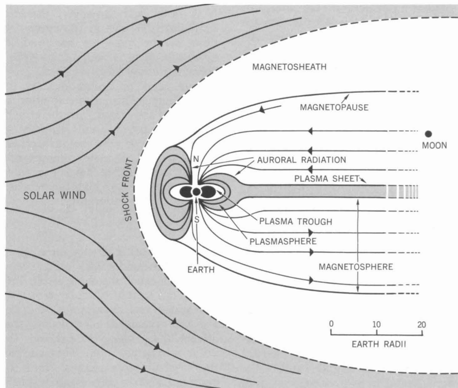
Figure I-3 — THE MAGNETOSPHERE
