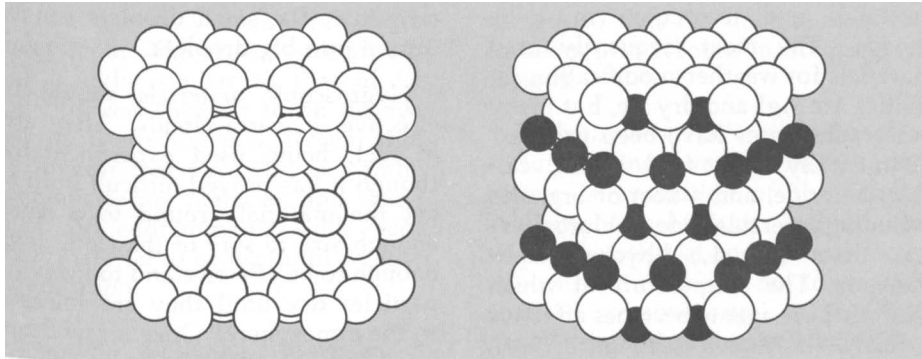
Figure VI-3 — LATTICE STRUCTURES OF AgI AND ICE
