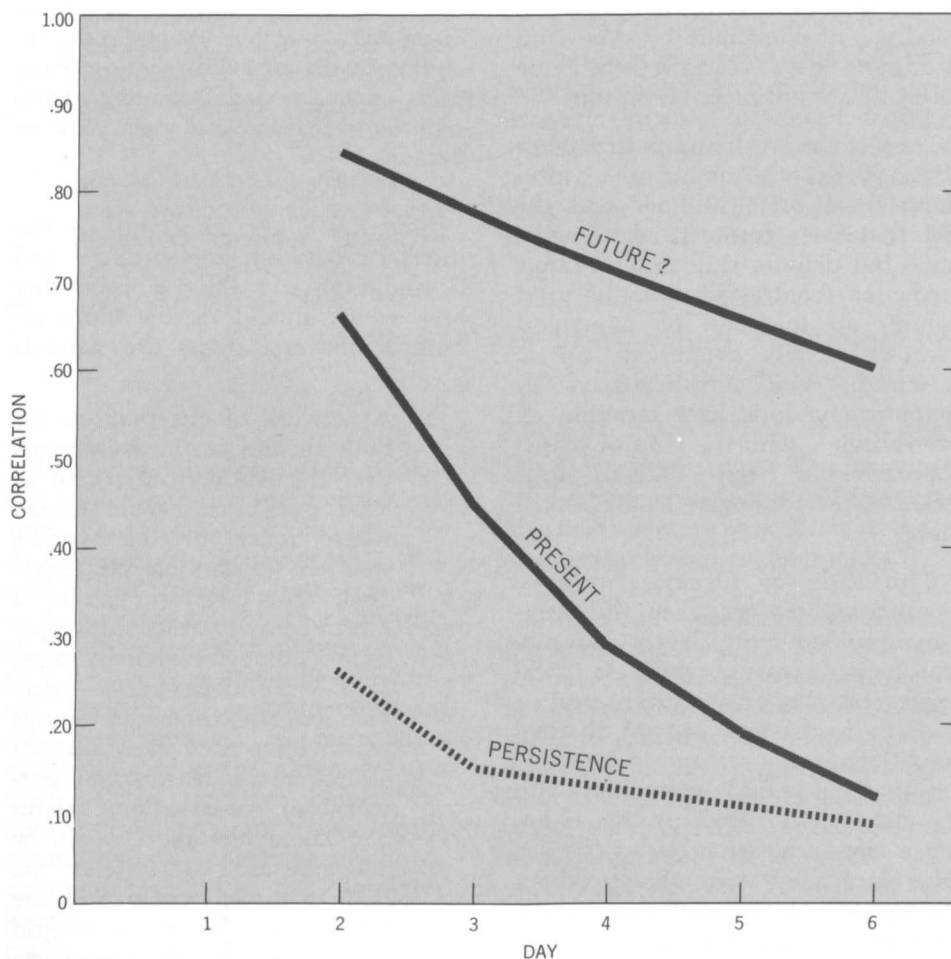
Figure IV-9 — FORECASTING SKILL
