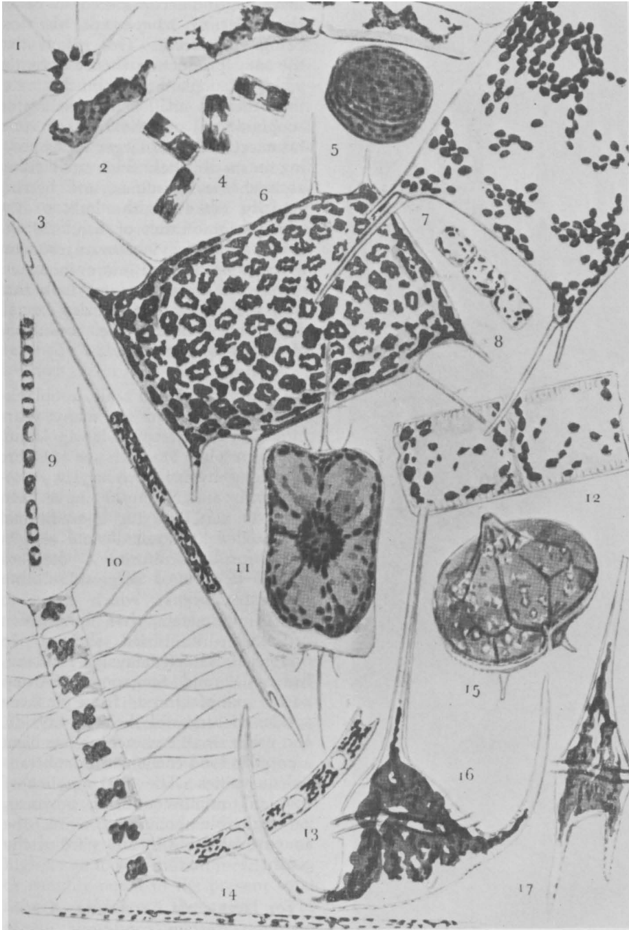
Figure VIII-4 — SOME PHYTOPLANKTON
