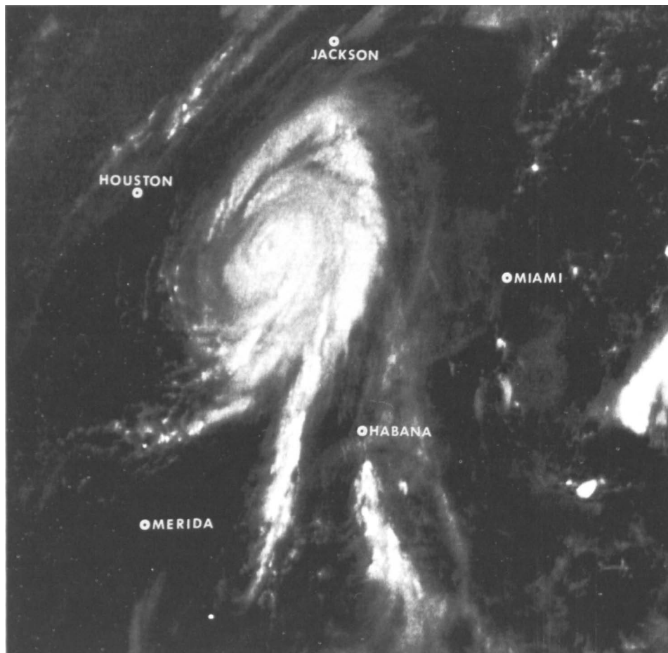
Figure V-5 — HURRICANE CAMILLE, 1969
