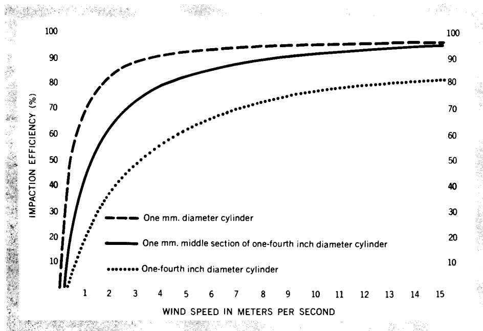
Figure X-10 — EFFICIENCY OF CYLINDRICAL COLLECTORS FOR RAGWEED POLLEN
