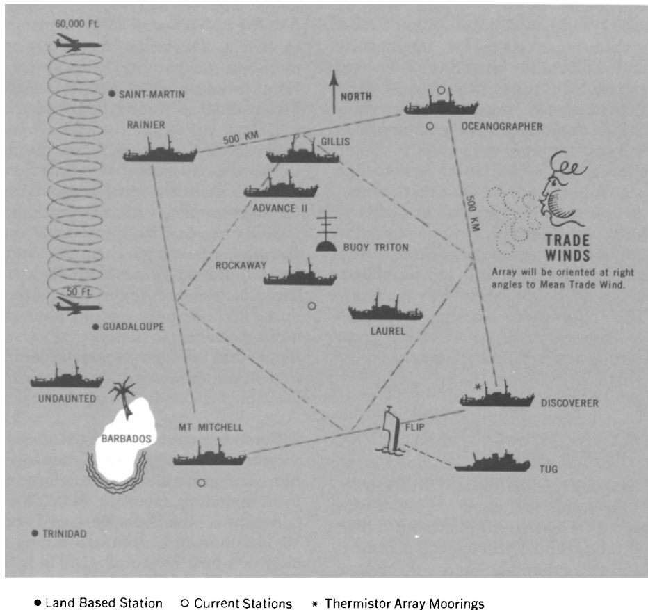
Figure VI-11 — ARRAY FOR BARBADOS OCEANOGRAPHIC AND METEOROLOGICAL EXPERIMENT (BOMEX)
