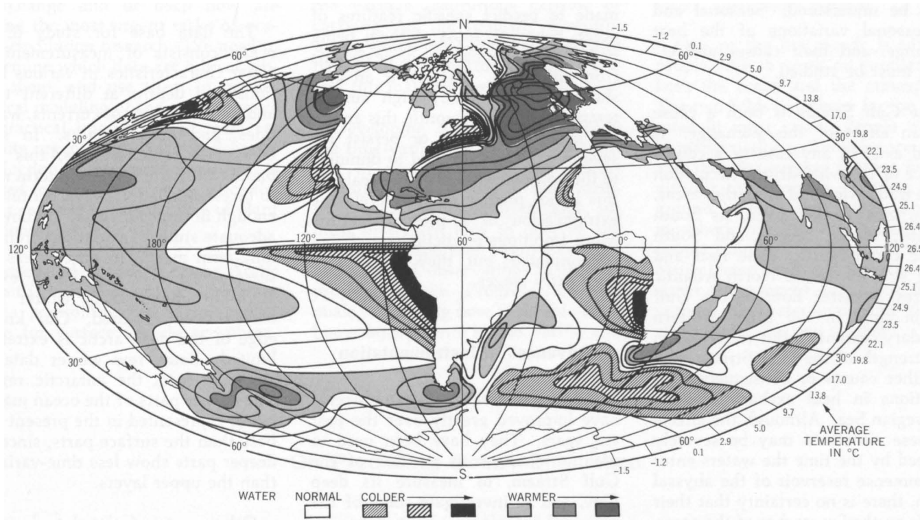
Figure IV-1 — SEA-SURFACE TEMPERATURE
