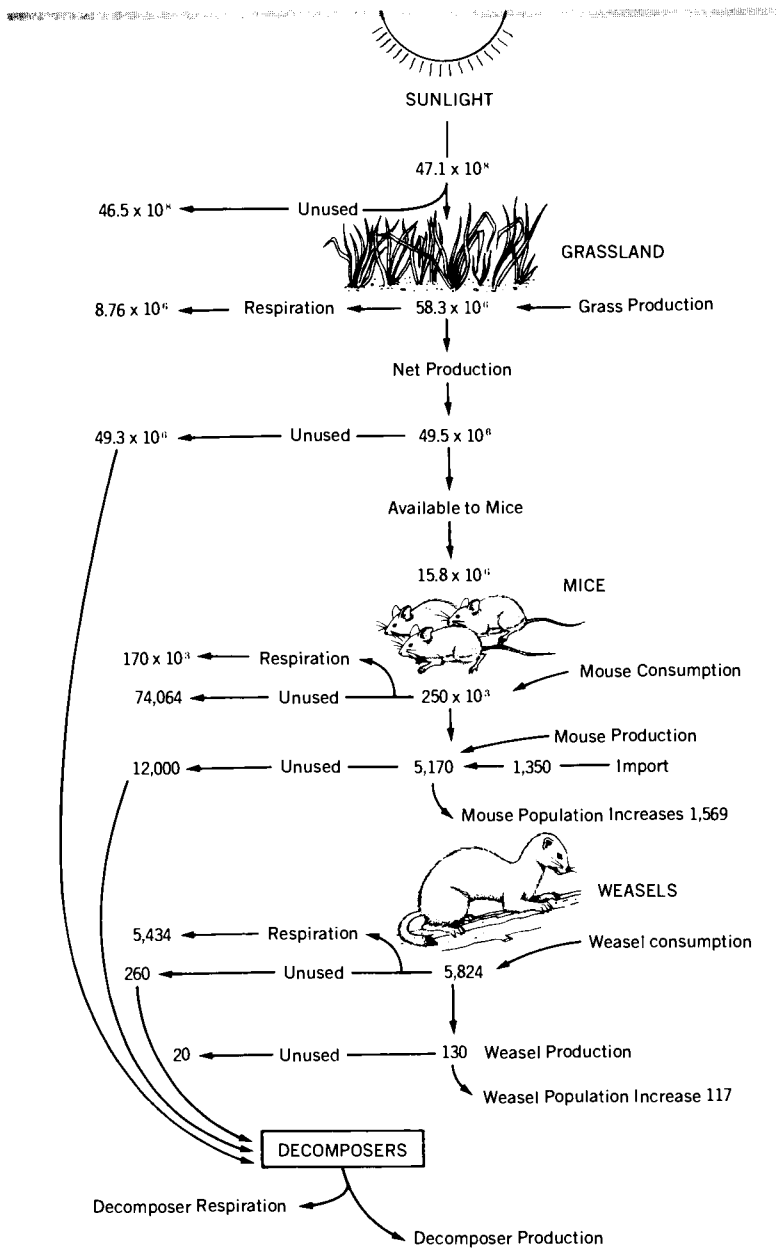
Figure IX-6 — PLANT-MOUSE-WEASEL CHAIN
