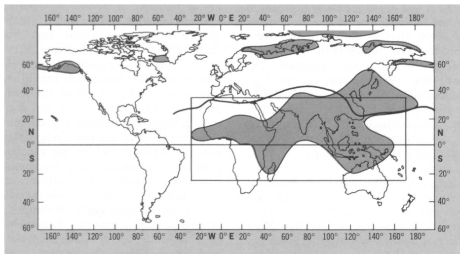
Figure VI-10 — MONSOONAL AREAS
