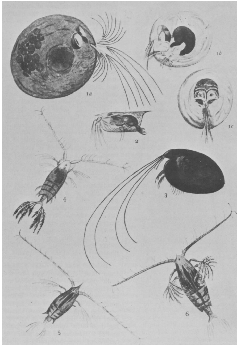
Figure VIII-5 — SOME ZOOPLANKTON
