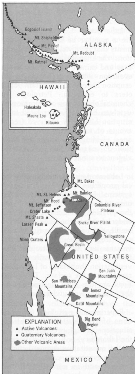
Figure II-8—U.S. VOLCANOES
