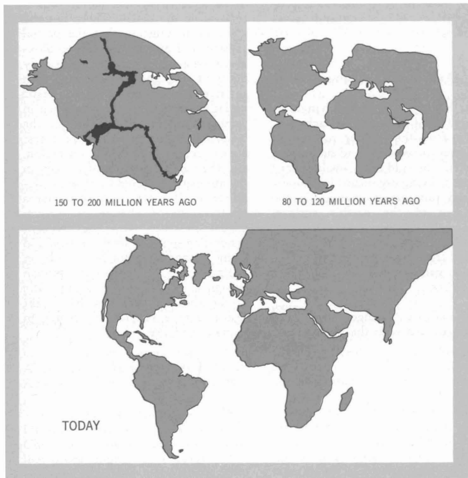
Figure II-4—CONTINENTAL DRIFT
